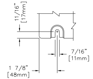
BOLT SLOT DETAIL QUARTER SCALE
